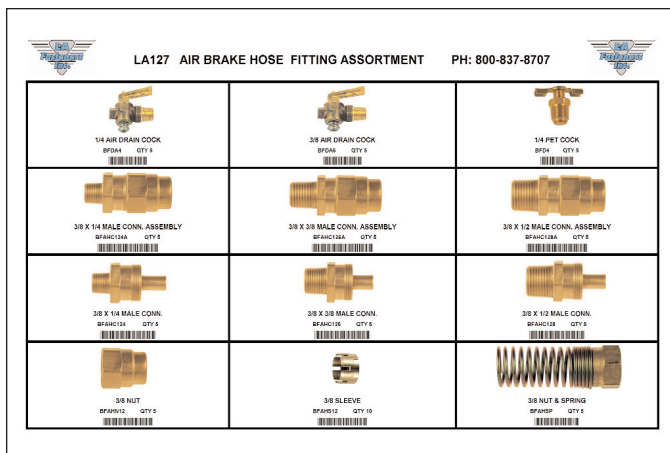
LA127 AIRBRAKE HOSE ASSORTMENT
